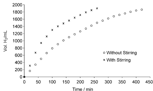
Figure 5. Solid-state solvolysis of 1 g of ammonia borane by catalyst 2 and water vapor ( 25^\circ C ).
