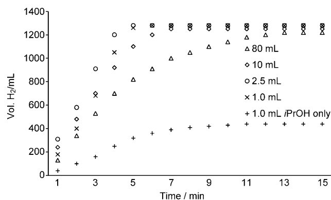
Figure 4. Effect of solvent volume on volume of H_2 produced in the solvolysis of ammonia borane with 2 in iPrOH/H_2O (1:1; v/v) at 40^\circ C .
